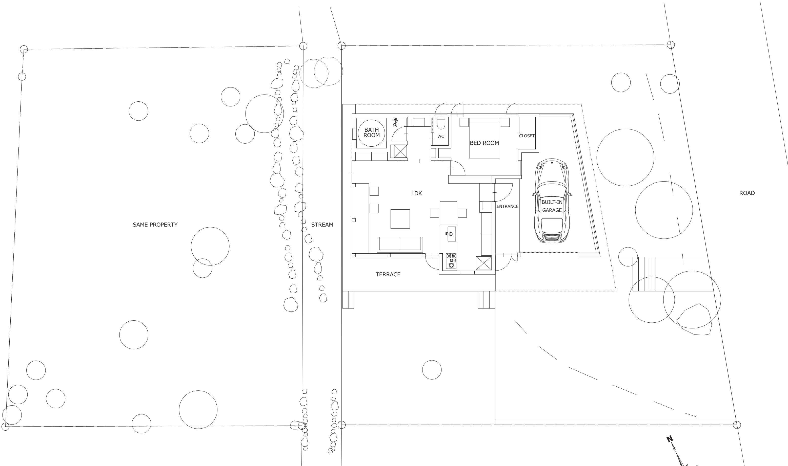
Layout Plan
